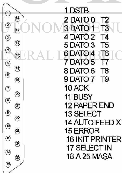
Figura 4.9. Puerto LPT1
