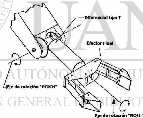
Figura 4.6: Efector final.
